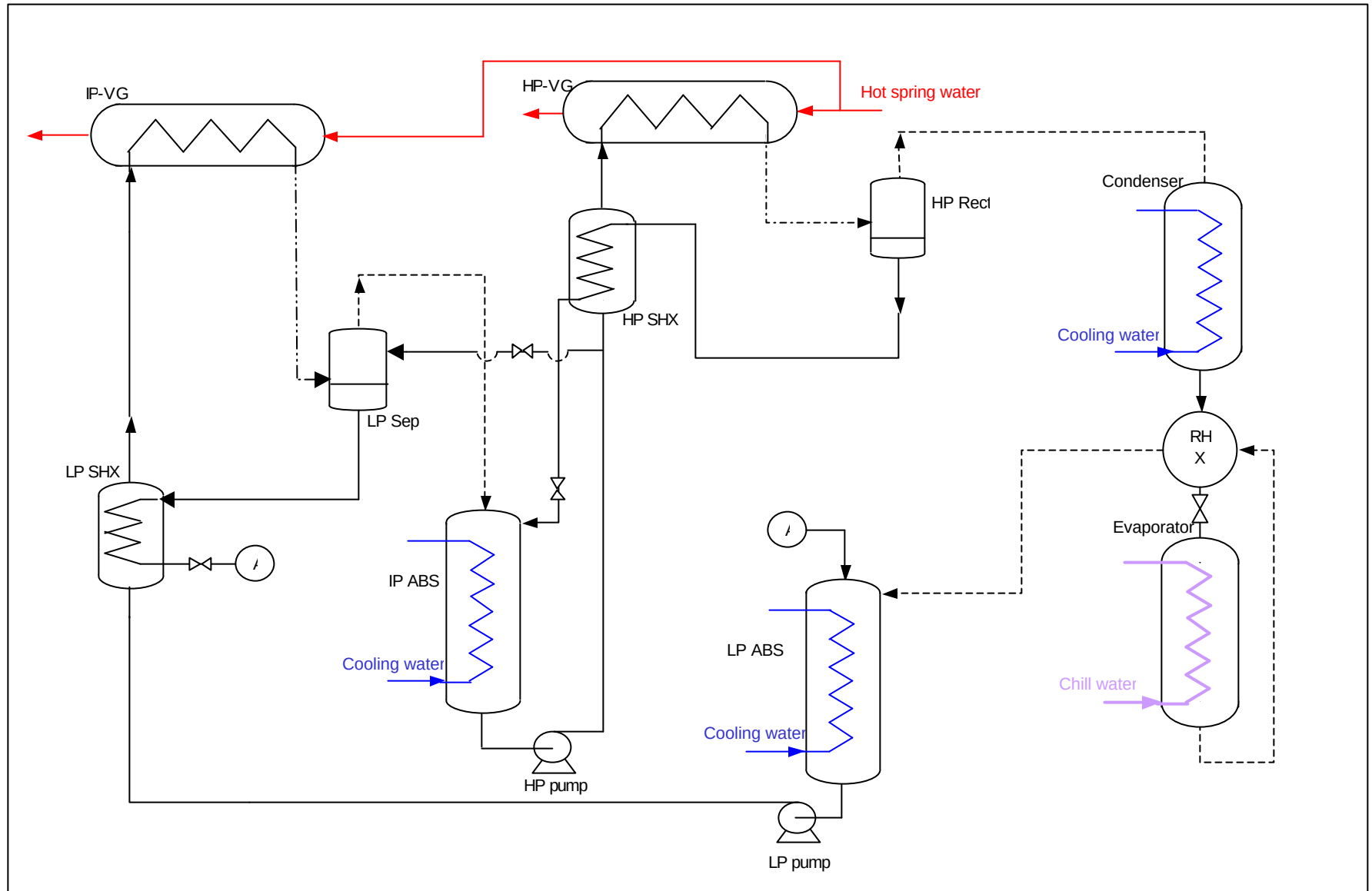
Fig. 1 Chena Hot Springs Double Lift (Three Pressure) Absorption Refrigeration Cycle
